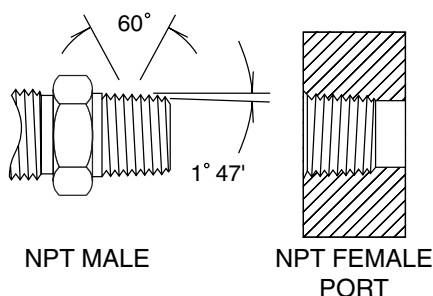
Figure 73: NPT (National Pipe Taper)
