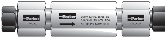
MAF Series Dual Disc Line Filter
