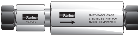
MAFC Series Cup Type Line Filter
